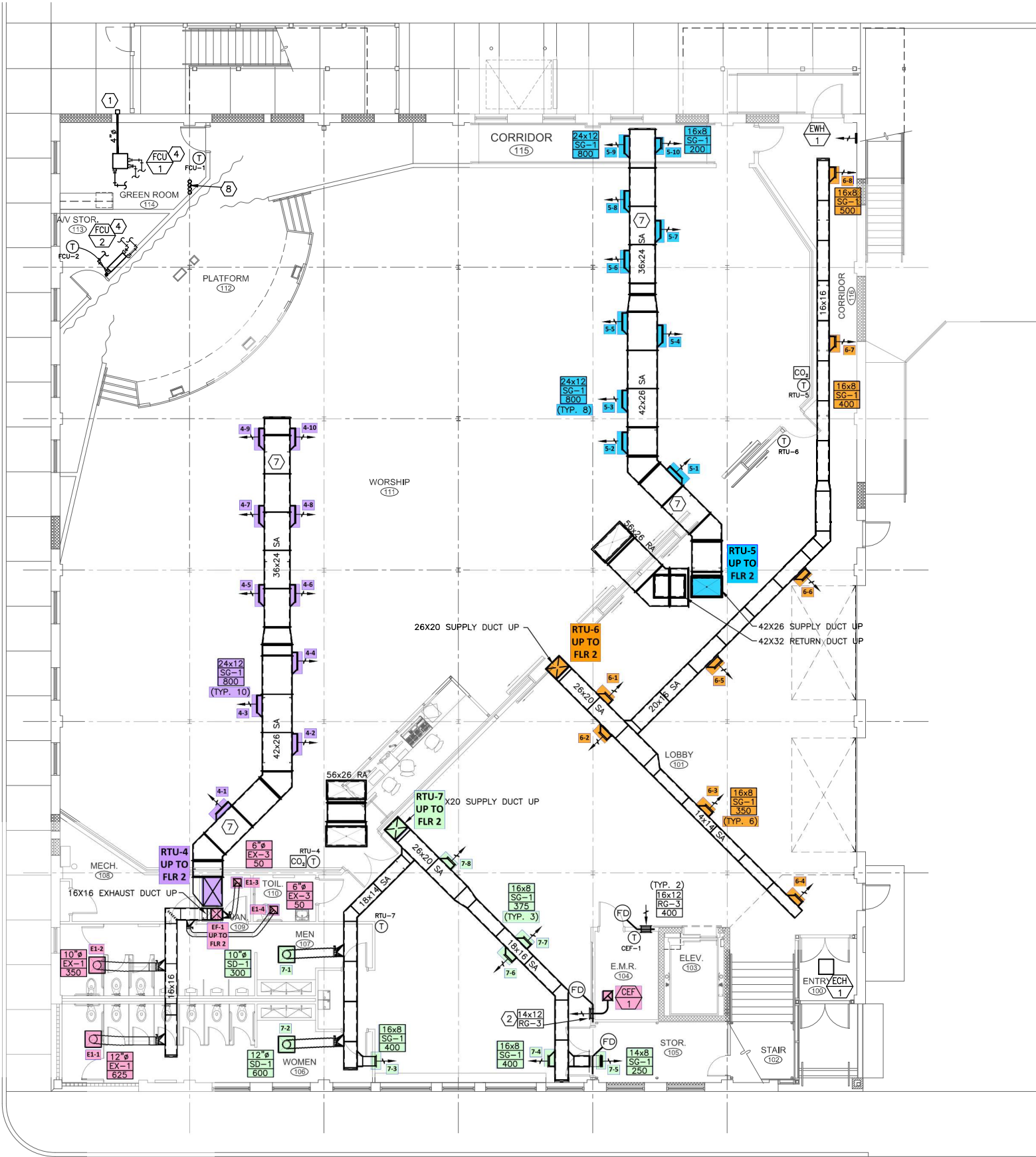
1 FIRST FLOOR MECHANICAL PLAN M1.10 SCALE: 1/8" = 1'-0"
